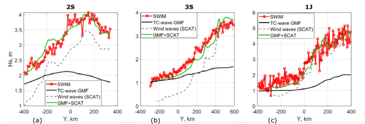
Figure 4. H_s profiles for tracks 2S (a), 3S (b) and 1J (c).
