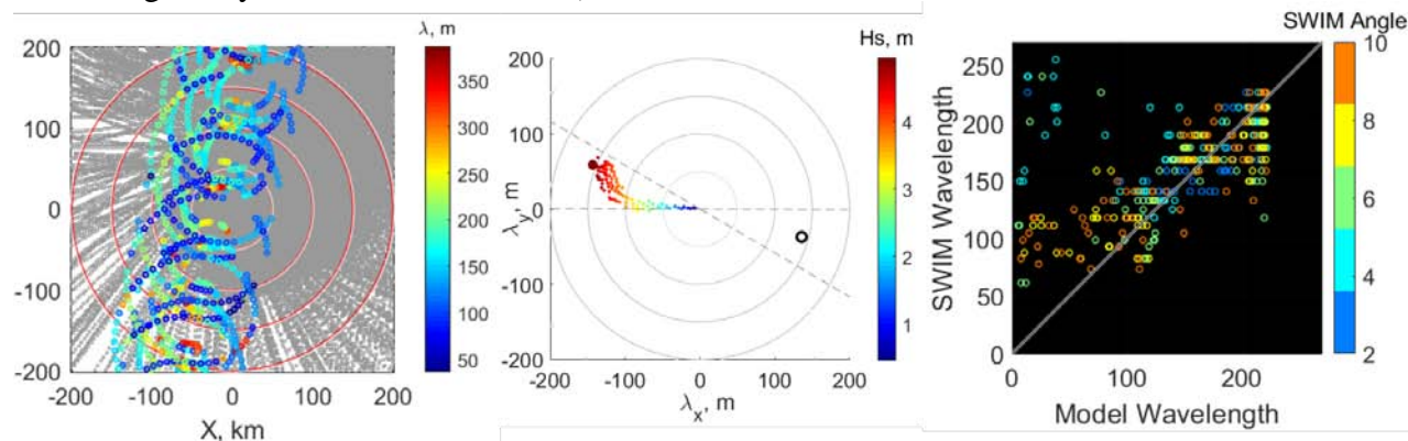
Figure 5. (Left) The modeled wave-rays (gray) and SWIM off-nadir measurements ( 2^\circ , 4^\circ , 6^\circ , 8^\circ , 10^\circ incidence angles). Color indicates the peak wavelength of 1D spectrum. (Center) SWIM and model wavelength comparison. Color dots: average characteristics of model wave rays in the vicinity of one SWIM beam acquisition (black circle). The wave-train with maximum wavelength is taken into account only in a case if its direction lies between the two dashed lines indicating \pm 15^\circ from SWIM observation azimuth. (Right) A scatter plot for all points satisfying the above criterion. Color is SWIM beam zenith angle.
