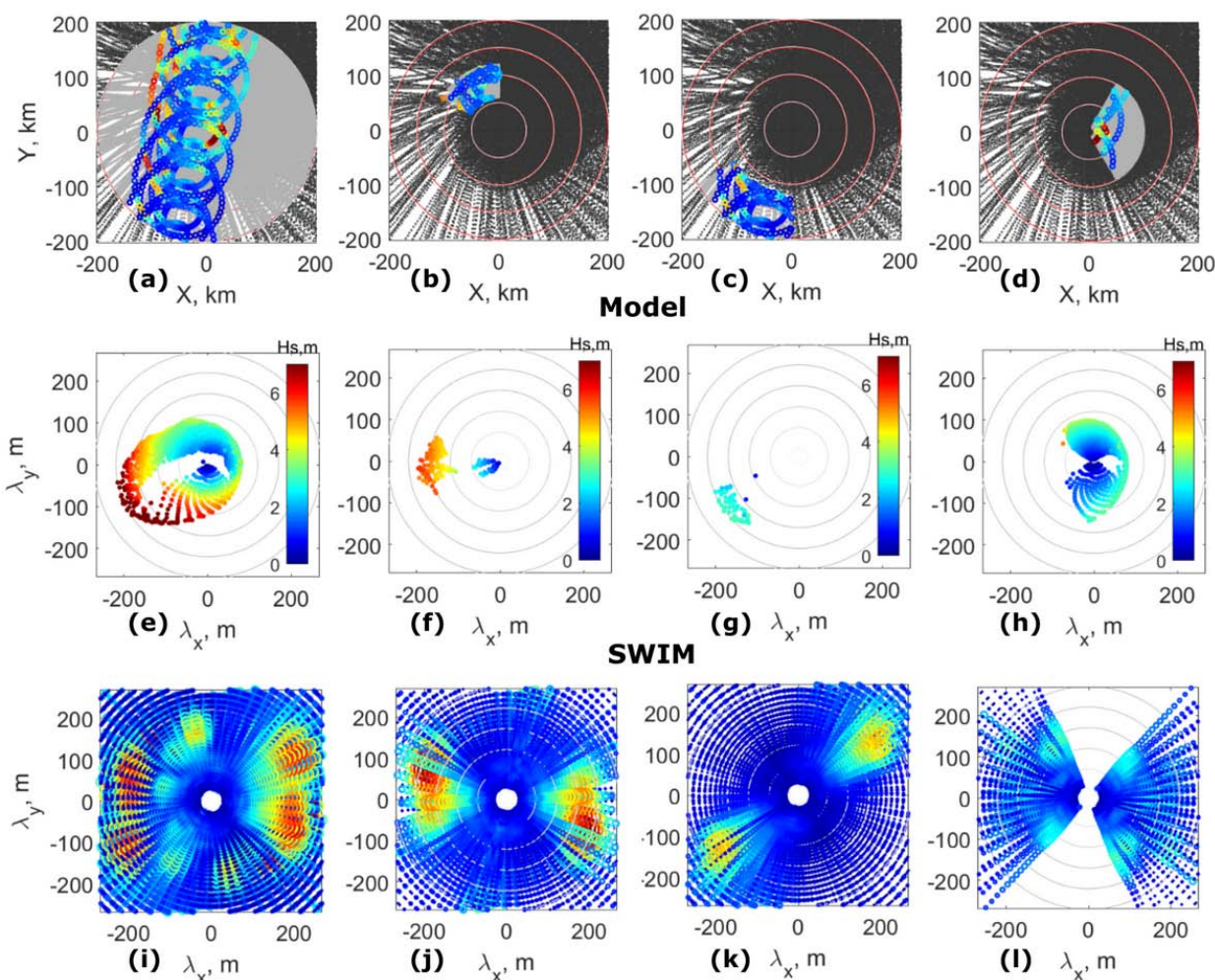
Figure 6. (a)-(c) The same as Fig. 4 (left) but for selected TC areas. (e)-(h) Characteristics of modeled wave-trains inside these areas (one point is one ray). (i)-(l) Superposition of SWIM 1D spectra for each beam in selected area.
