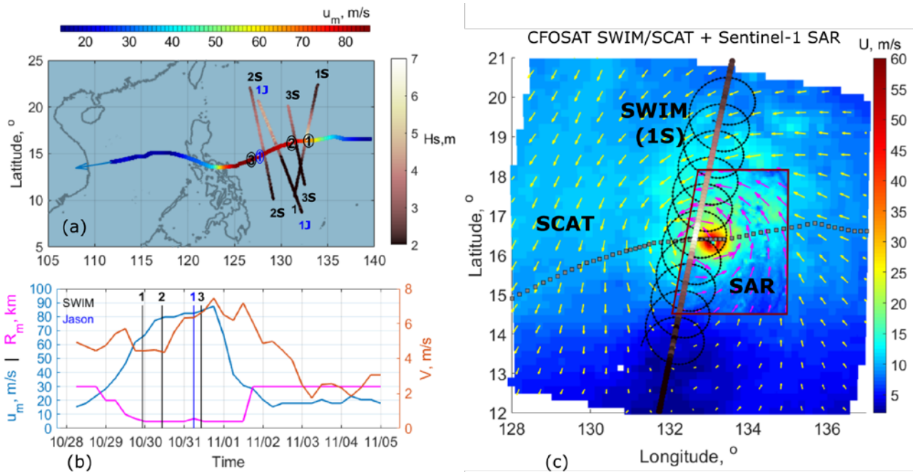
Figure 1. (a) TC Goni track and Hs altimeter measurements. Circled numbers indicate TC location at time of satellite passage. (b) Time evolution of Goni parameters. (c) Wind fields from CFOSAT SCAT and Sentinel-1A SAR data (outlined polygon), TC track (gray squares), CFOSAT SWIM nadir Hs (the same colormap as on subplot (a)) and SWIM rotating beam track with 10° incidence
