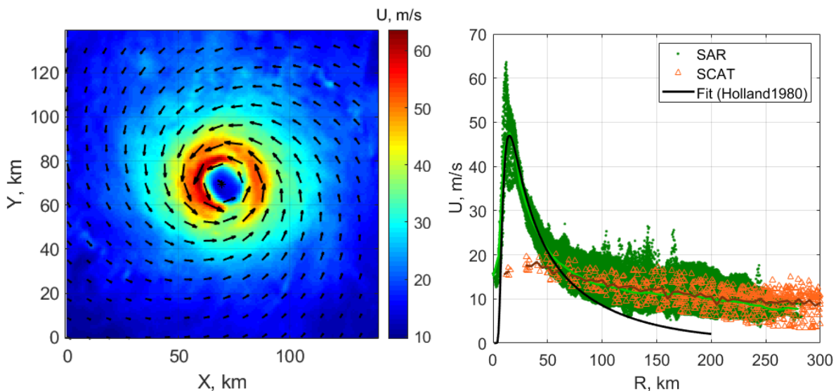
Figure 2. (a) Wind field inside TC Goni retrieved from Sentinel-1 SAR. (b) Wind speed profiles from SAR (green) and CFOSAT SCAT (orange) data. Solid lines are respective 5 km-binned
